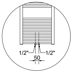
Detail of the 50 mm pipe centres version.
